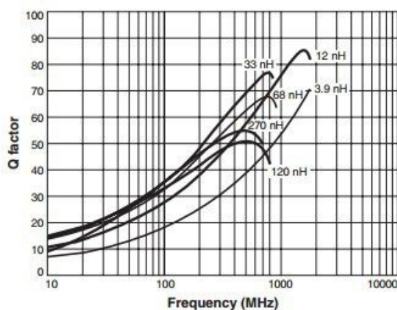
Typical Q vs Frequency
