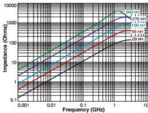
Typical Impedance vs Frequency
