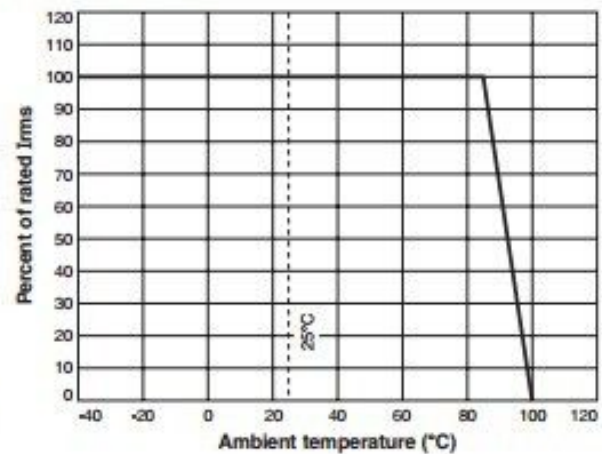
Irms Derating
